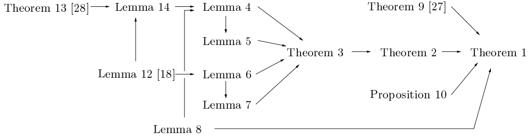
FIGURE 1. Proof of Theorem 1 - Flowchart
