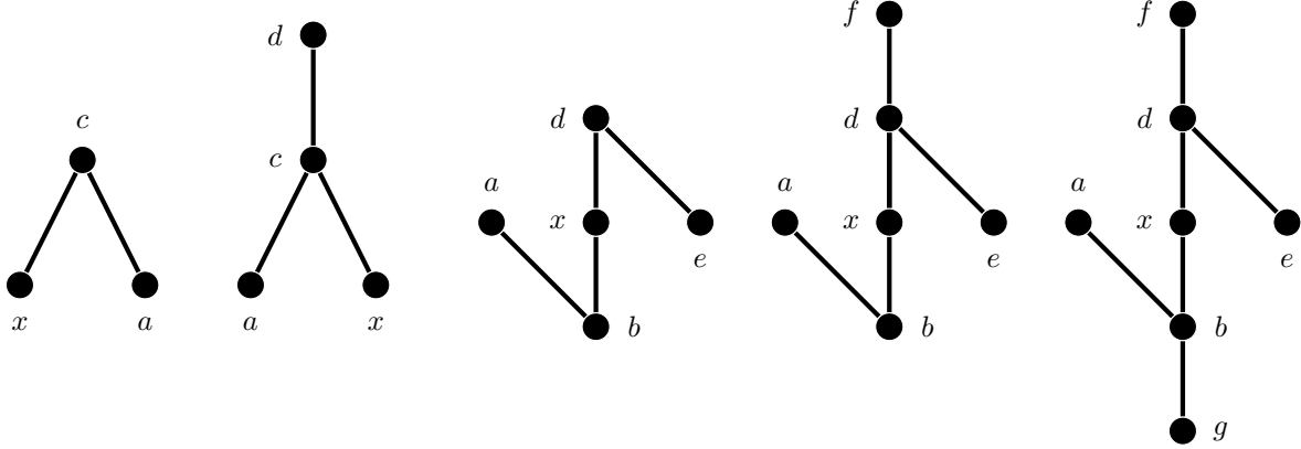
FIGURE 3. The Hasse diagrams of the \wedge , Y^d , \mathcal{S} , \mathcal{S}^+ , and \mathcal{S}^{++} posets.
