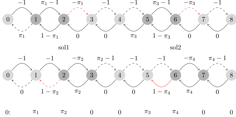
FIGURE 7. The case of two solitons: “dangerous” edges
