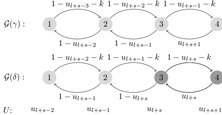
FIGURE 3. Case (C2): head of a soliton. Cycle (3,4) of \mathcal{G}(\delta) is critical
