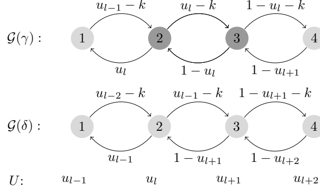
FIGURE 2. Case (C2): tail of a soliton. Cycle (2,3) of \mathcal{G}(\gamma) is critical.
