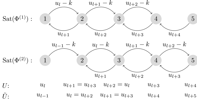
FIGURE 4. Undressing in (C1)
