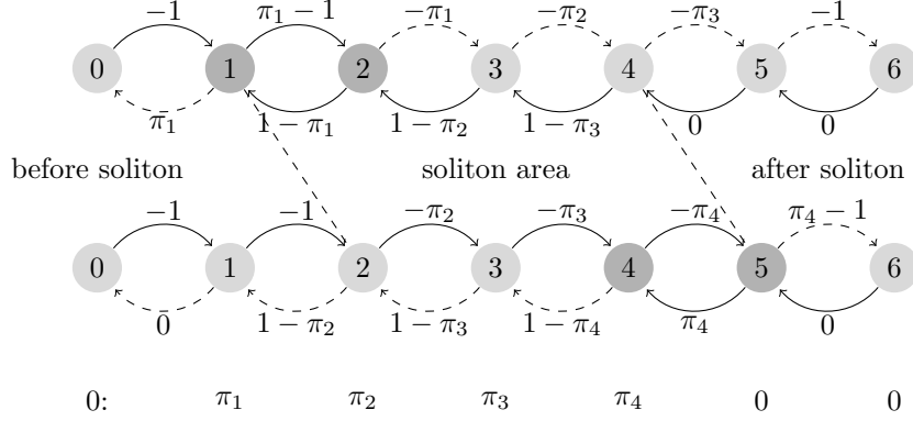
FIGURE 6. The case of one soliton
