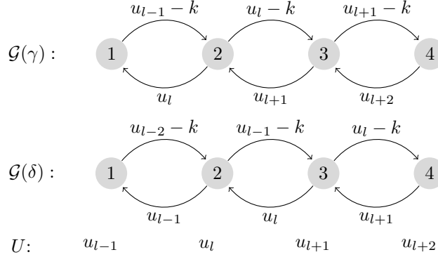
FIGURE 1. Case (C1): a fragment of the associated digraphs
