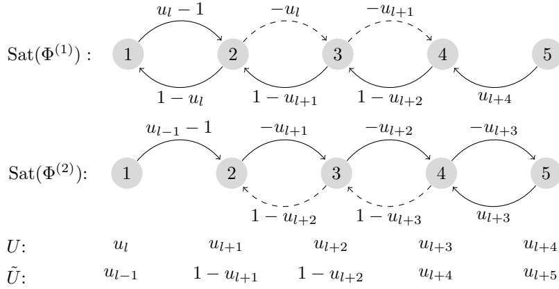
FIGURE 5. Undressing in (C2). The dashed edges indicate that they belong to saturation graphs if and only if u_i + u_{i+1} = 1 for the corresponding i , that is, if the two-cycle containing them is critical.
